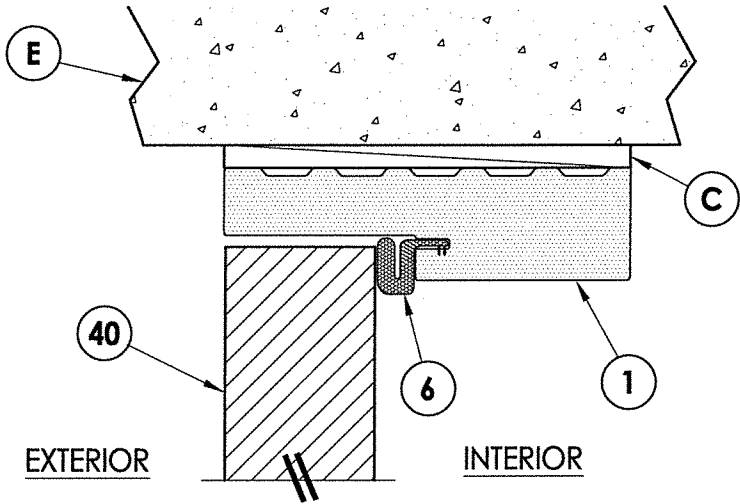
1 5 VERTICAL CROSS SECTION Outswing shown (Inswing similar)
